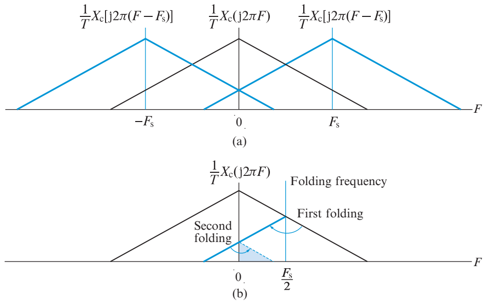
Figure 6.14 Aliasing distortion can be equivalently explained (a) by considering the overlapping tails of shifted replicas of the input spectrum, or (b) by folding the right tail of the input spectrum about F_s/2 and zero until the entire tail is in the range 0 \leq F \leq F_s/2 .
