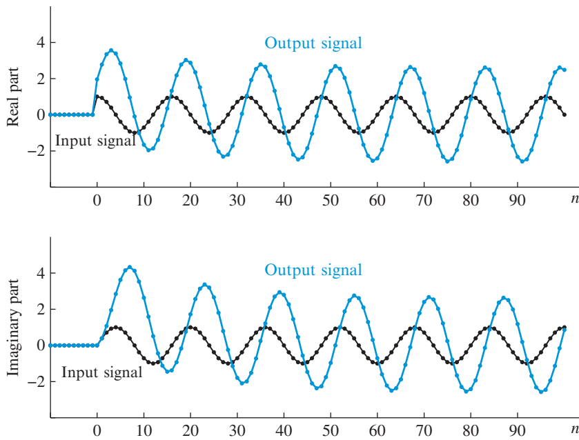
Figure 2.27 Transient and steady-state responses to a suddenly applied complex exponential sequence.
