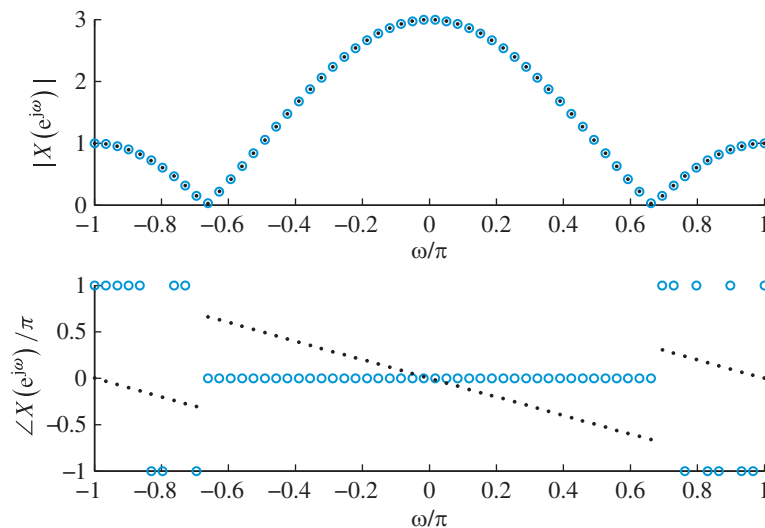
Figure 4.25 Computation of the DTFT of x[n] = \delta[n+1] + \delta[n] + \delta[n-1] using MATLAB functions freqz ( \cdot ) and dtft12 ( \circ ), respectively.
