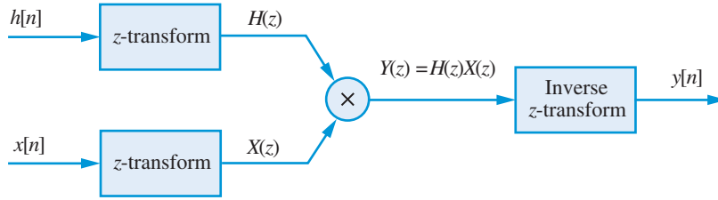
Figure 3.7 Procedure for the analytical computation of the output of an LTI system using the convolution theorem of the z -transform.
