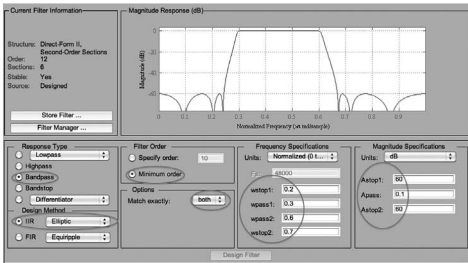
Figure 11.39 FDATool user interface for the design of a digital elliptic bandpass filter used in Example 11.25.
