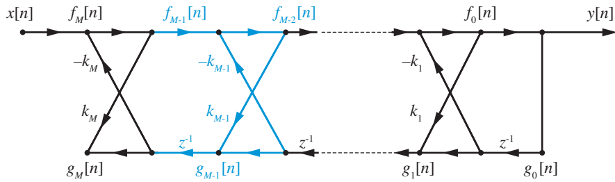
Figure 9.27 An all-pole lattice structure.
