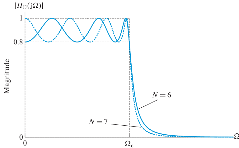
Figure 11.9 Magnitude responses of two Chebyshev I lowpass filters with ripple parameter \epsilon = 0.75 and orders N = 6 (solid-line) and N = 7 (dashed-line).
