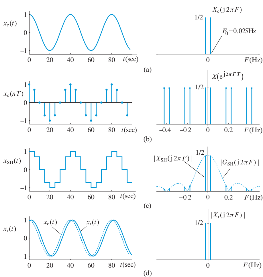
Figure 6.28 Frequency domain characteristics of S/H reconstruction. F_s = 0.2 \text{ Hz} .
