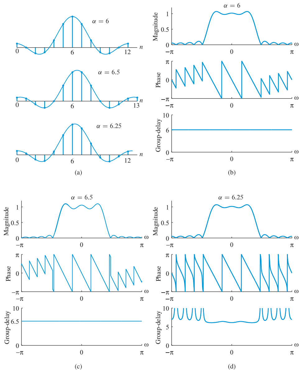
Figure 10.2 (a) Impulse responses of ideal analog lowpass filter with \omega_c = 0.4\pi and delays of \alpha = 6 , 6.5, and 6.25, respectively, along with samples of the truncated ideal lowpass FIR filter impulse response. Shown are magnitude response, phase response, and group delay of the truncated ideal lowpass FIR filter with (b) \alpha = 6 and M = 12 , (c) \alpha = 6.5 and M = 13 , and (d) \alpha = 6.25 and M = 13 . Observe that if 2\alpha is not an integer, then the phase response is nonlinear and the group delay is not a constant.
