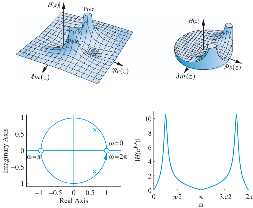
Figure 4.26 The relationship between the z -transform and the DTFT for a sequence with two complex-conjugate poles at z = 0.9e^{j\pi/4} and two zeros at z = \pm 1 .
